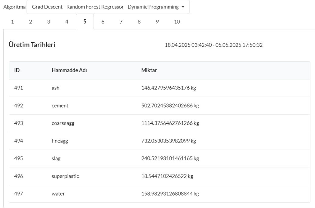
Figure 7.37 System Output 37
