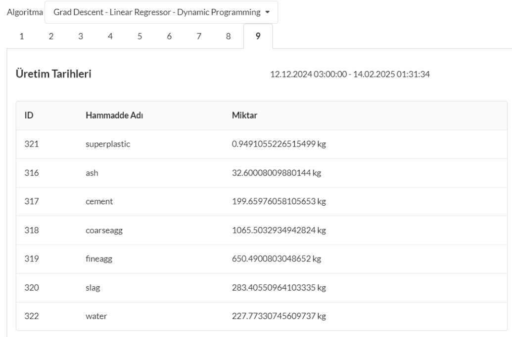
Figure 7.12 System Output 12
